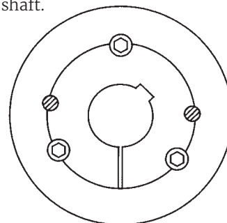
Bush with 3 Grub Screws (Sizes 3535 and above)
