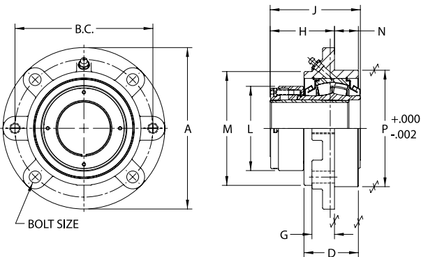
USFCE5000A Series Flange Cartridge Units - Adapter Mount, Type E Mounting Dimensions
