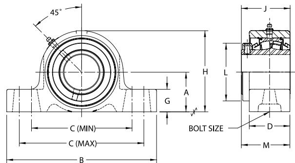
USRBE5000 Series Two-Bolt Base Pillow Blocks - Collar Mount, Type E Mounting Dimensions
