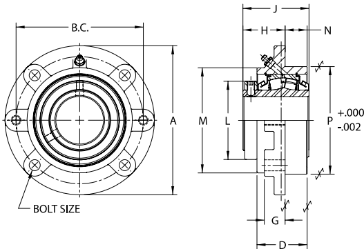
USFCE5000 Series Flange Cartridge Units - Collar Mount, Type E Mounting Dimensions
