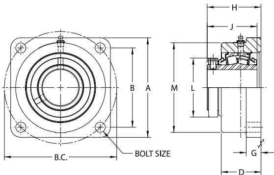
USFBE5000 Series Four-Bolt Flange Units - Collar Mount, Type E Mounting Dimensions
