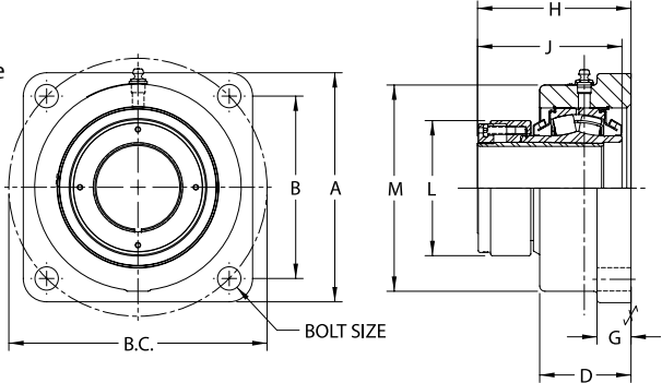
USFBE5000A Series Four-Bolt Flange Units - Adapter Mount, Type E Mounting Dimensions
