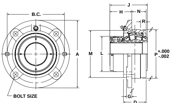
Mid-Spherical Bearings
